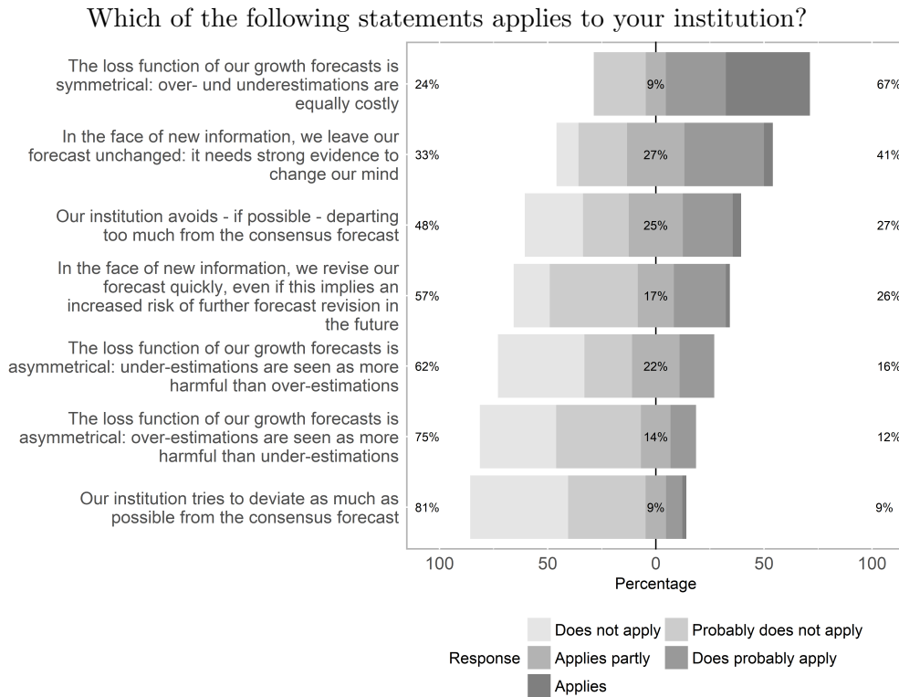
Figure 8: Attitudes to Consensus and Loss Functions
