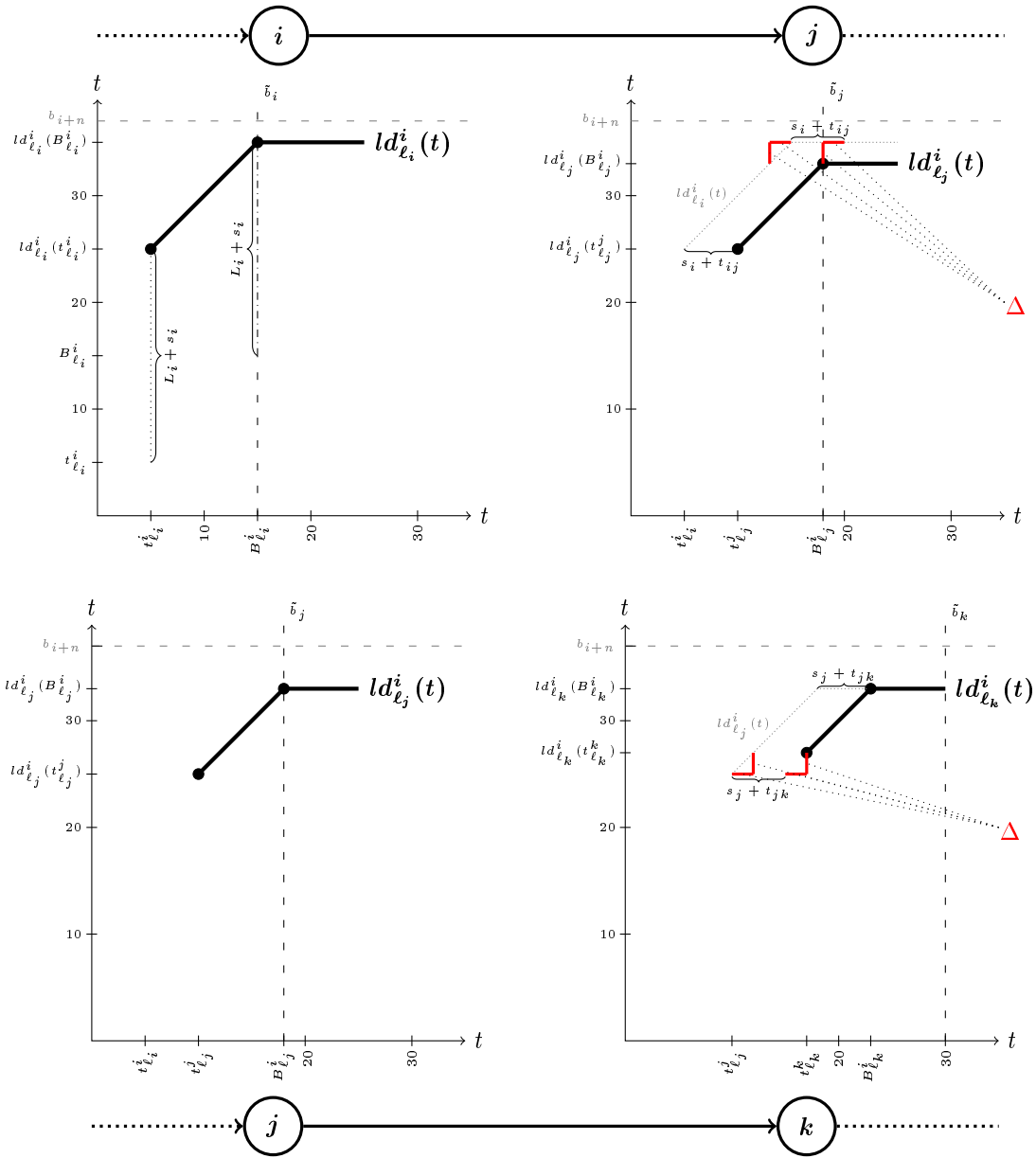
Figure 2: Extension of labels: Latest delivery times ld^i(t) for an open request i for the extension along arc (i, j) (upper part) and along arc (j, k) (lower part)
